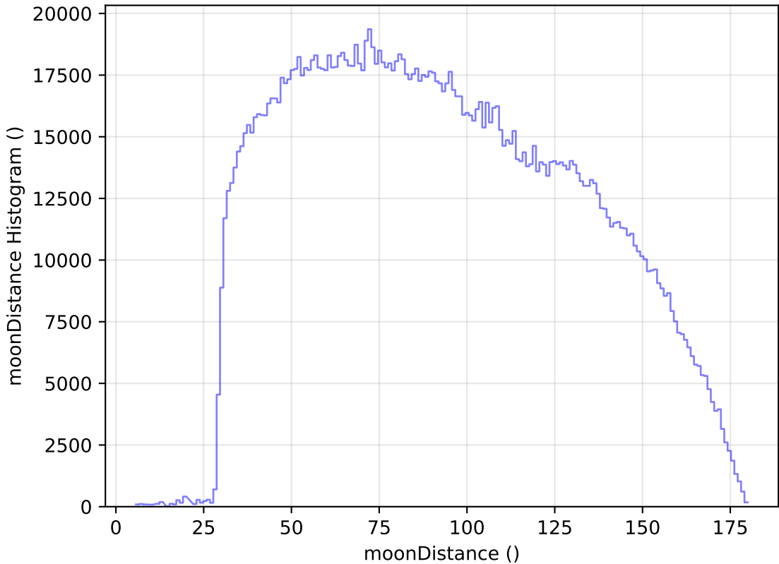
extra_ss_neo4_v3.4_10yrs WFD all bands: moonDistance Histogram
