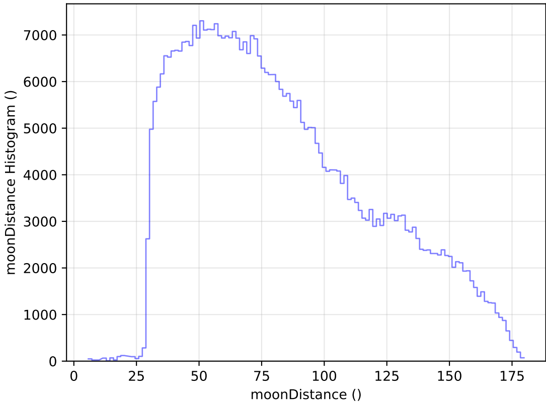
extra_ss_neo4_v3.4_10yrs All sky z band: moonDistance Histogram
