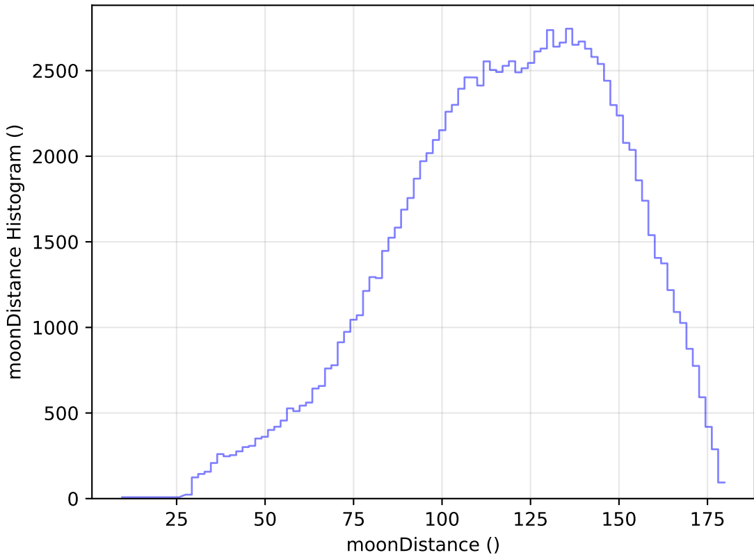
extra_ss_neo4_v3.4_10yrs All sky u band: moonDistance Histogram
