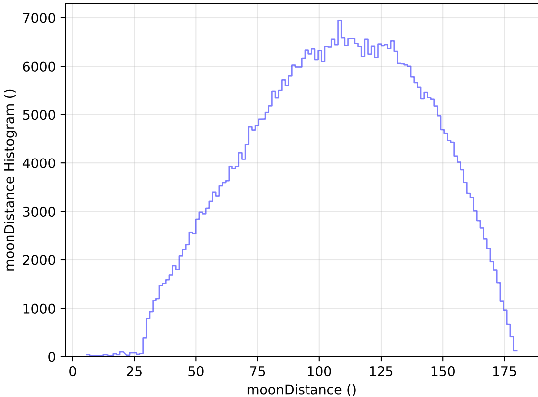
extra_ss_neo4_v3.4_10yrs All sky r band: moonDistance Histogram
