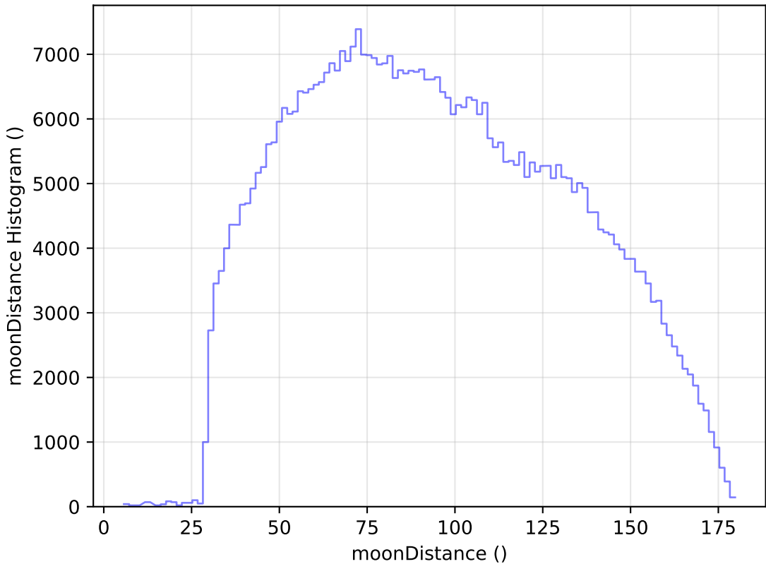
extra_ss_neo4_v3.4_10yrs All sky i band: moonDistance Histogram
