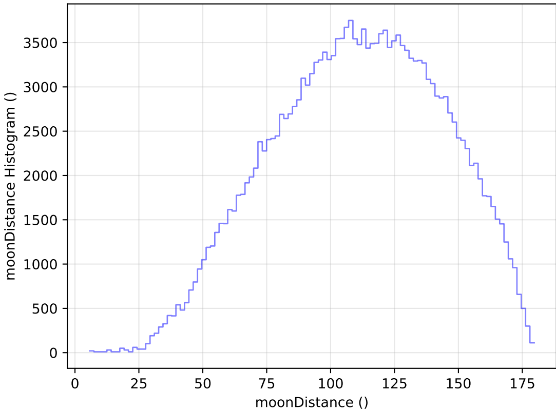
extra_ss_neo4_v3.4_10yrs All sky g band: moonDistance Histogram
