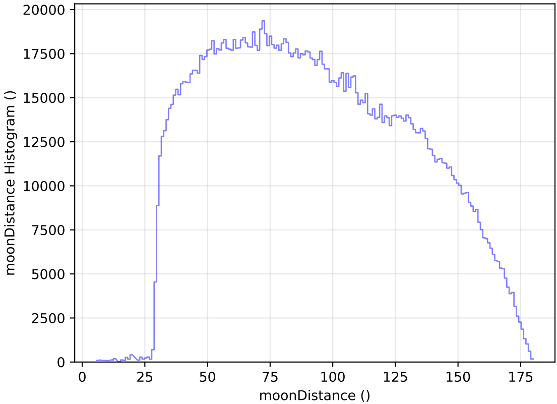
extra_ss_neo4_v3.4_10yrs All sky all bands: moonDistance Histogram
