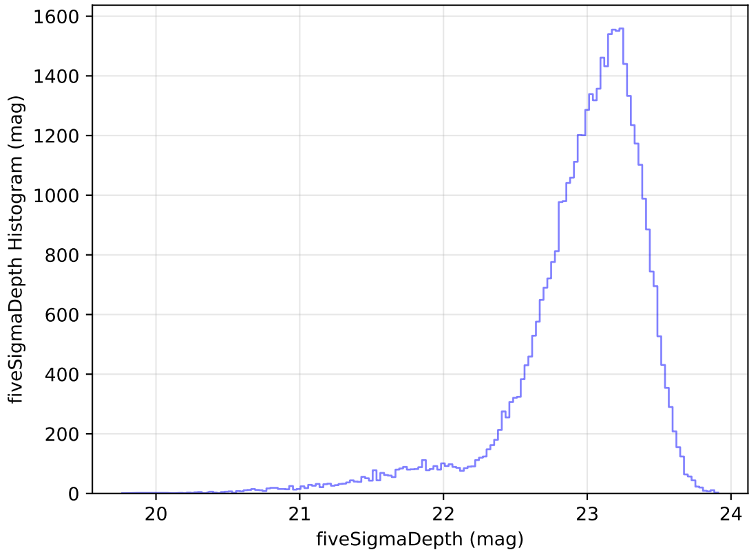
extra_ss_neo4_v3.4_10yrs Yr 1 z band: fiveSigmaDepth Histogram
