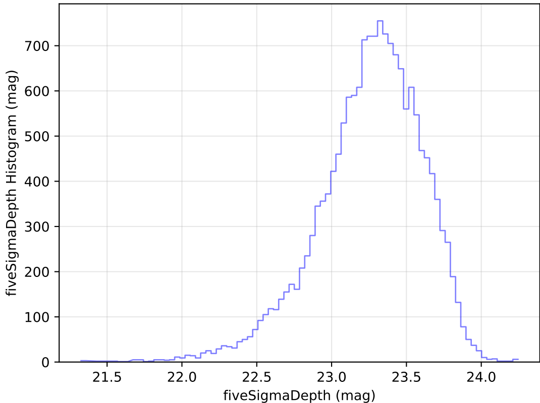
extra_ss_neo4_v3.4_10yrs Yr 1 u band: fiveSigmaDepth Histogram
