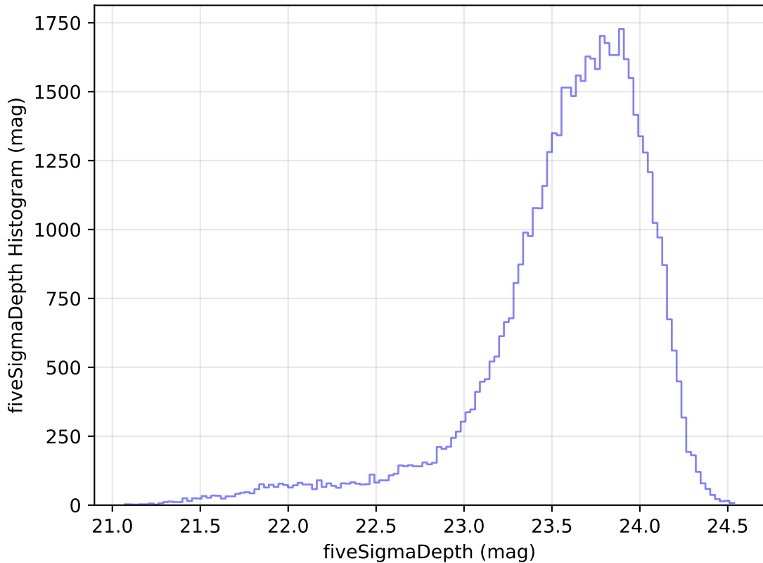
extra_ss_neo4_v3.4_10yrs Yr 1 i band: fiveSigmaDepth Histogram
