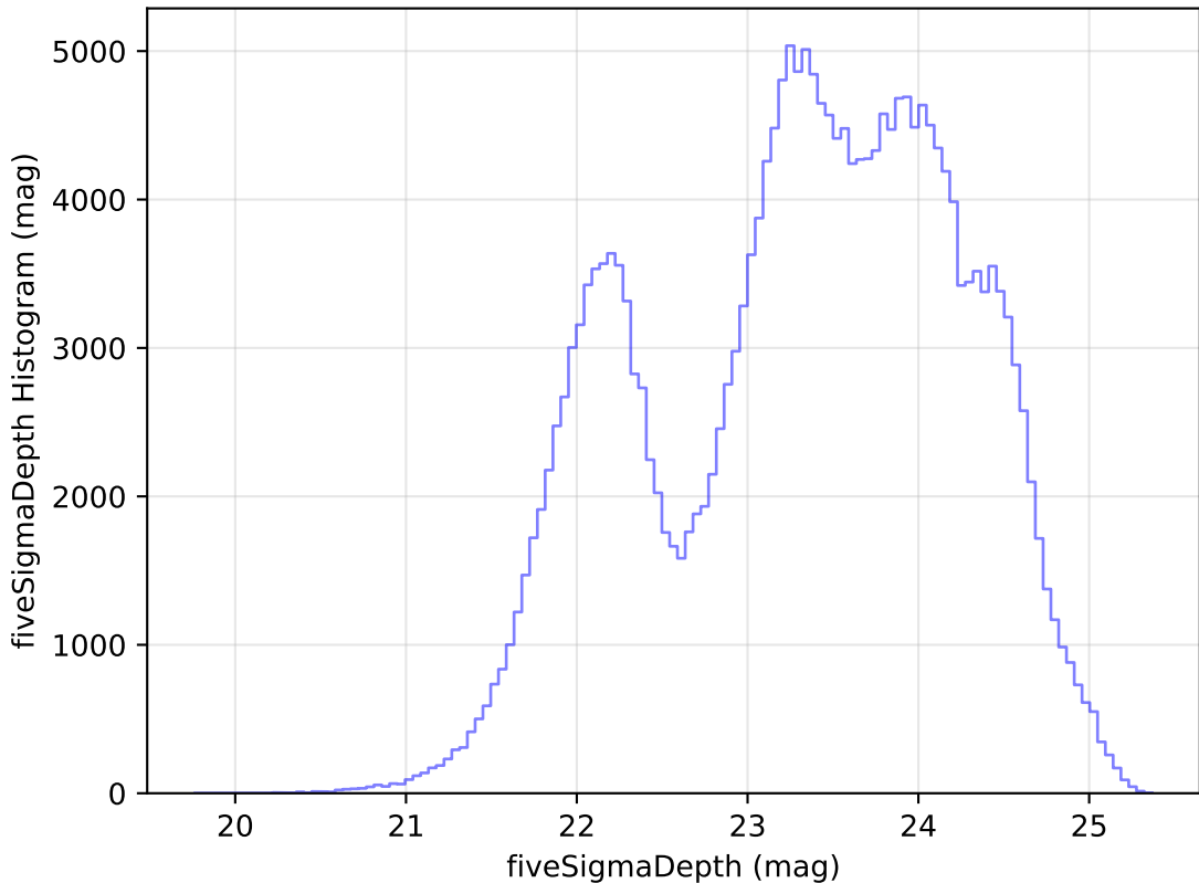
extra_ss_neo4_v3.4_10yrs Yr 1 all bands: fiveSigmaDepth Histogram
