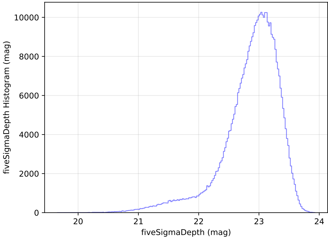
extra_ss_neo4_v3.4_10yrs WFD z band: fiveSigmaDepth Histogram
