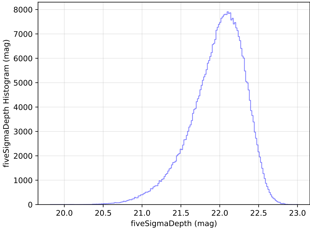
extra_ss_neo4_v3.4_10yrs WFD y band: fiveSigmaDepth Histogram
