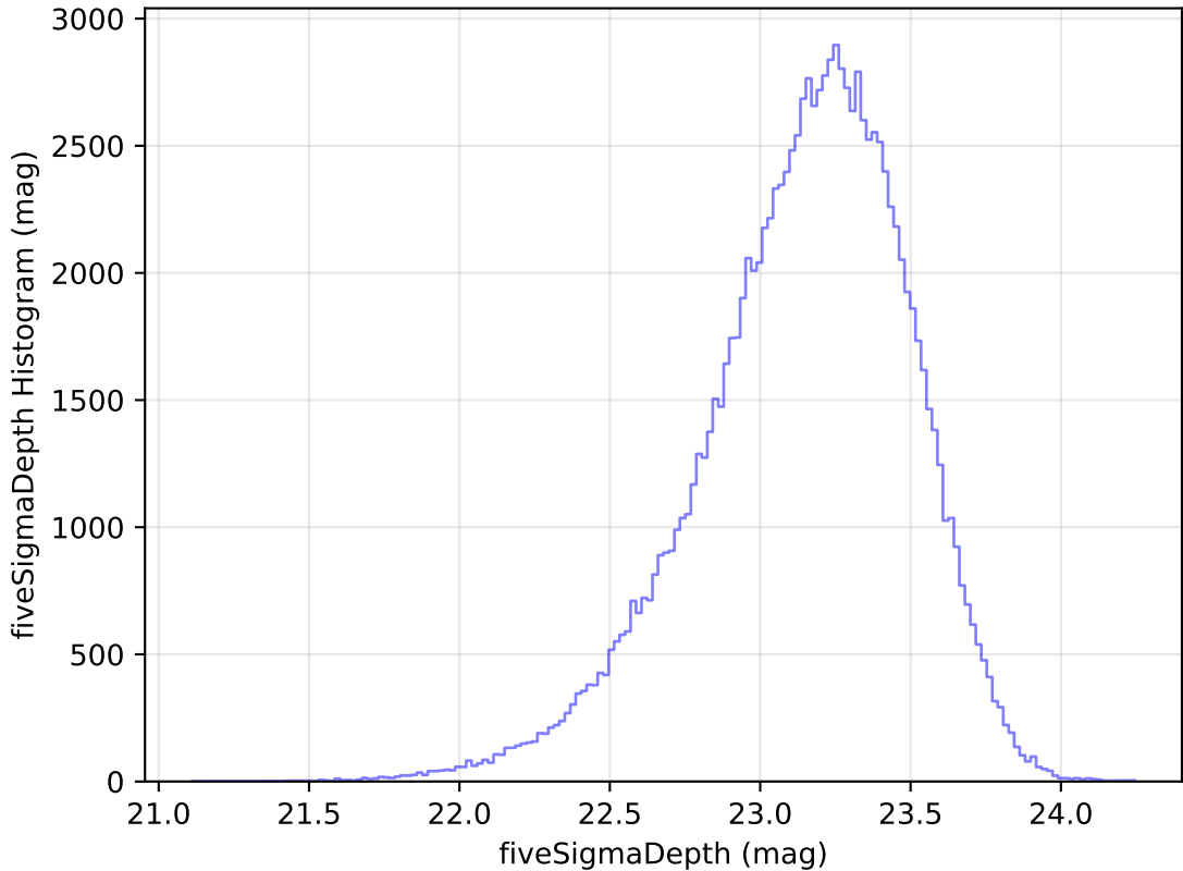
extra_ss_neo4_v3.4_10yrs WFD u band: fiveSigmaDepth Histogram
