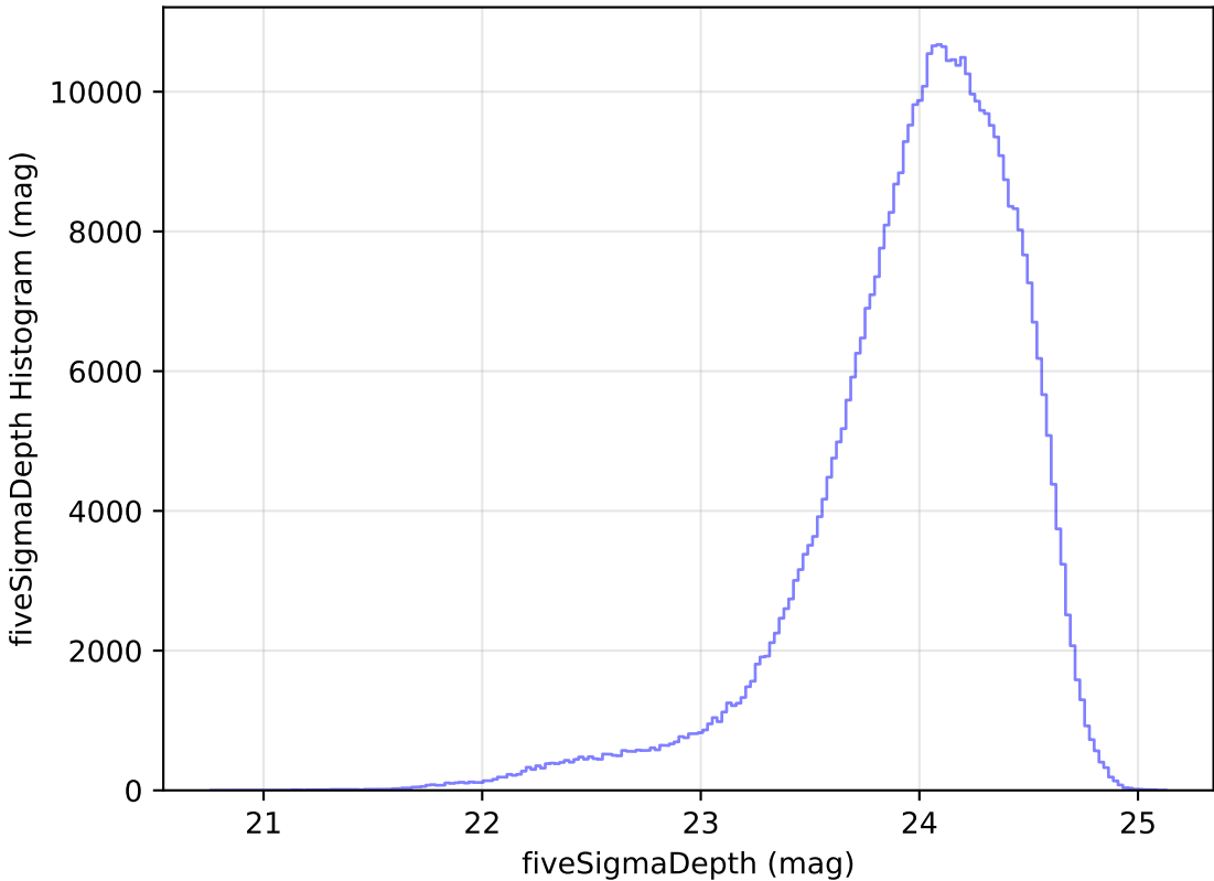
extra_ss_neo4_v3.4_10yrs WFD r band: fiveSigmaDepth Histogram
