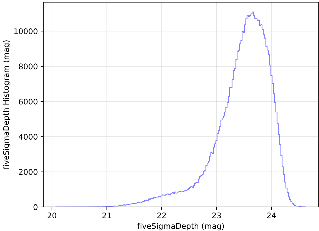
extra_ss_neo4_v3.4_10yrs WFD i band: fiveSigmaDepth Histogram
