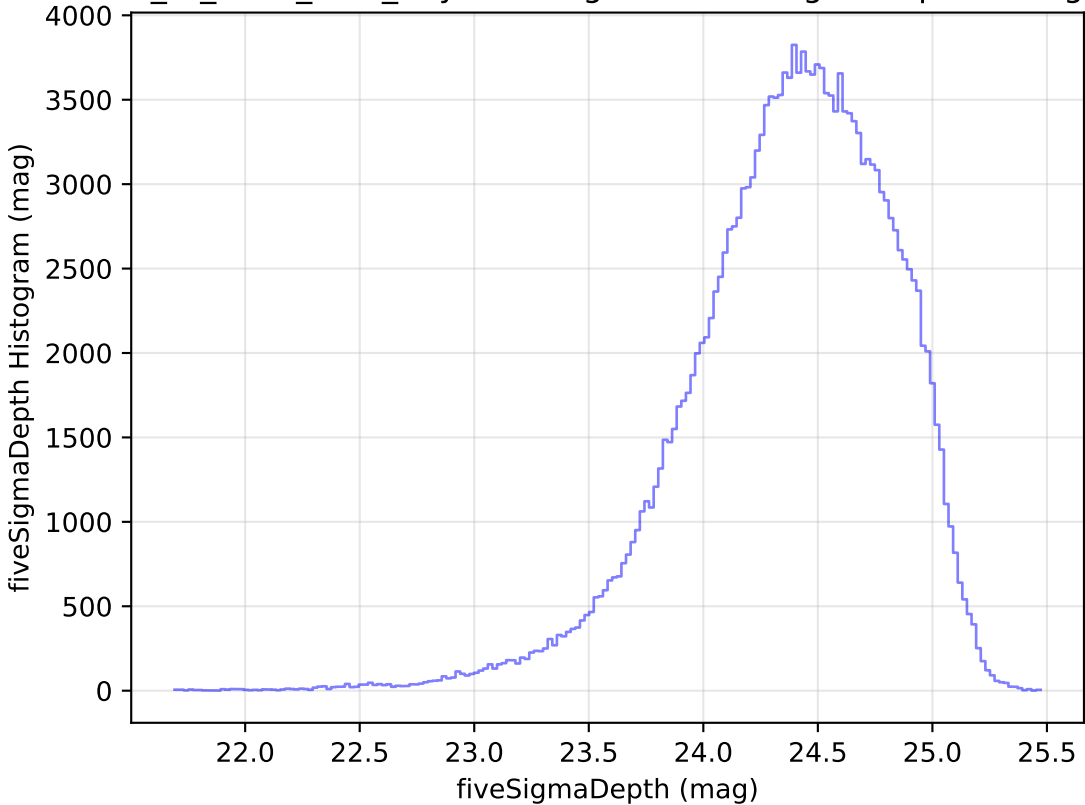
extra_ss_neo4_v3.4_10yrs WFD g band: fiveSigmaDepth Histogram
