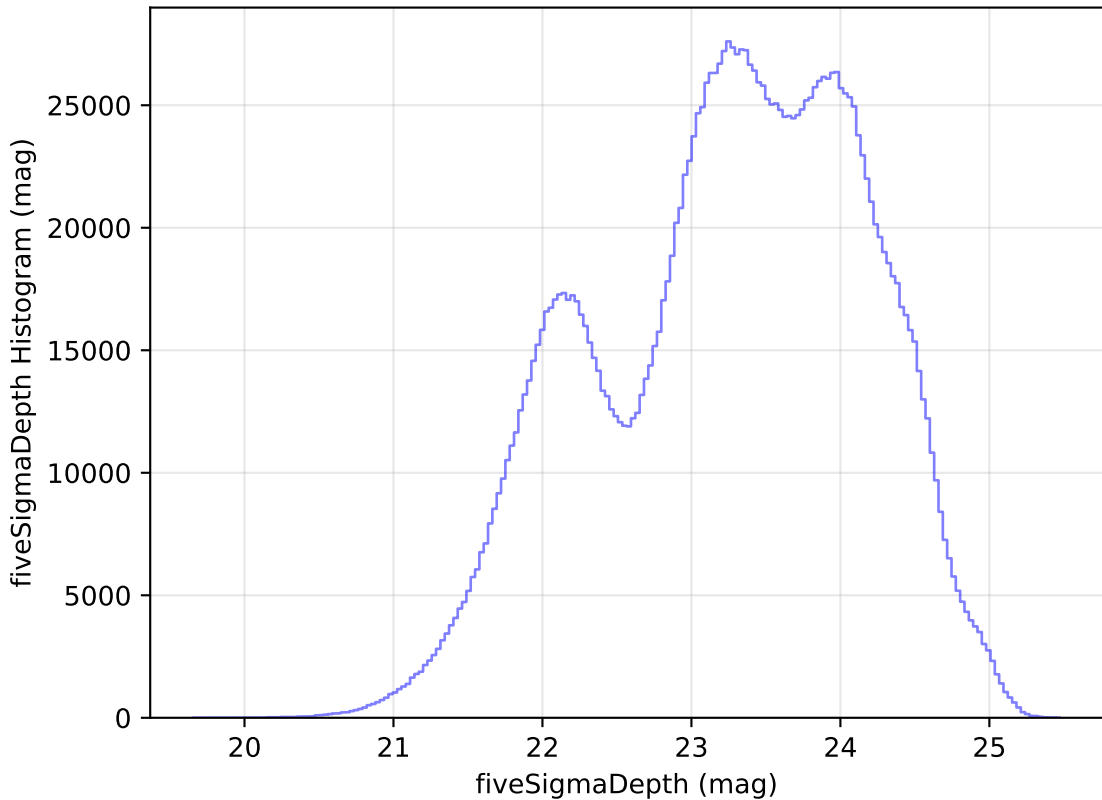
extra_ss_neo4_v3.4_10yrs WFD all bands: fiveSigmaDepth Histogram
