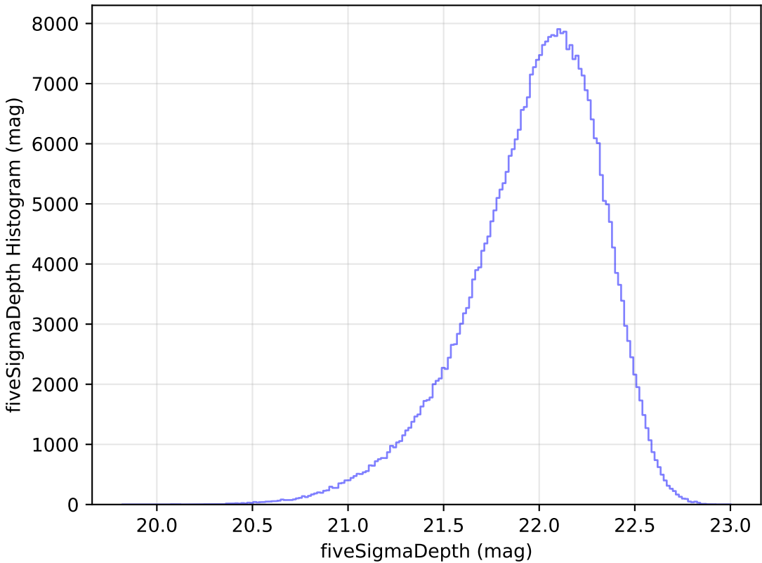
extra_ss_neo4_v3.4_10yrs All sky y band: fiveSigmaDepth Histogram
