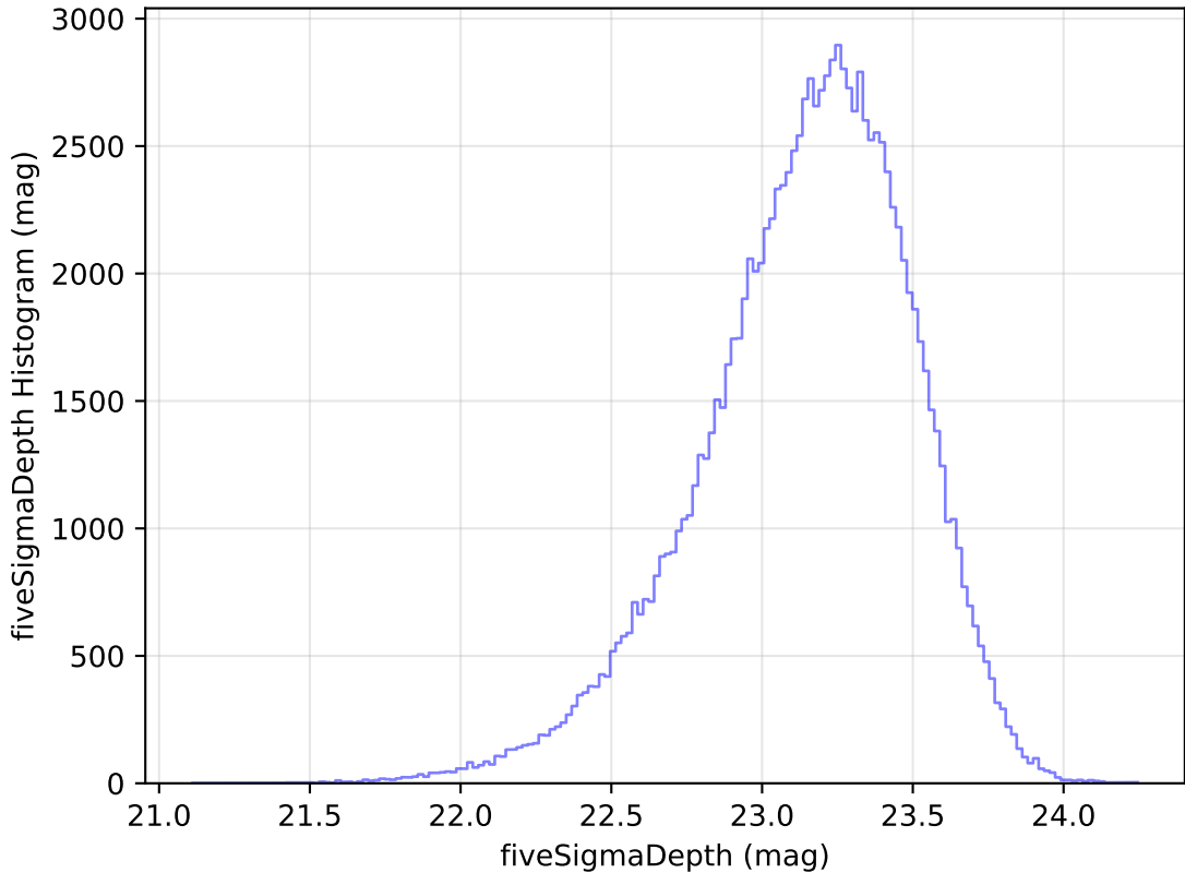
extra_ss_neo4_v3.4_10yrs All sky u band: fiveSigmaDepth Histogram
