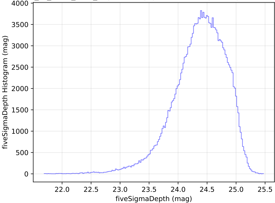
extra_ss_neo4_v3.4_10yrs All sky g band: fiveSigmaDepth Histogram
