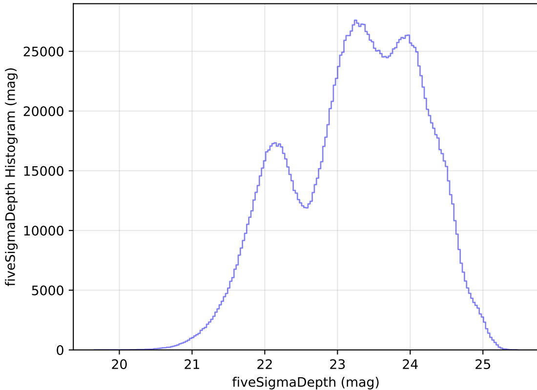
extra_ss_neo4_v3.4_10yrs All sky all bands: fiveSigmaDepth Histogram
