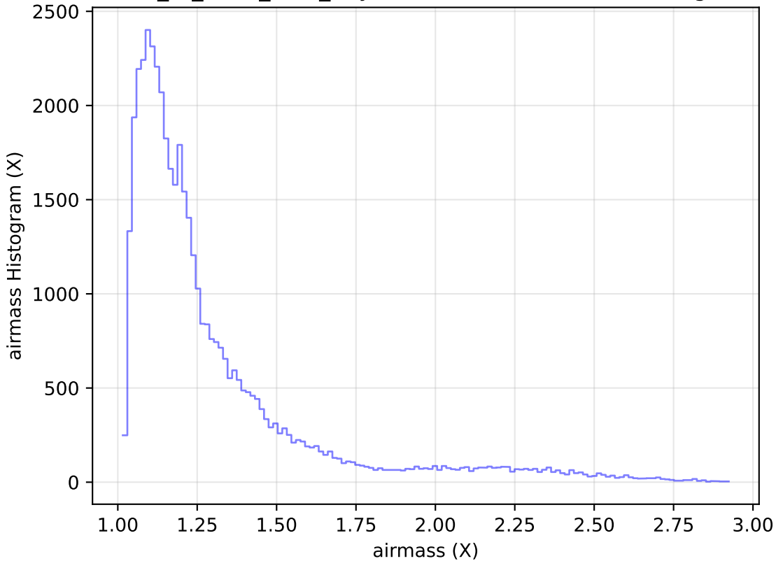
extra_ss_neo4_v3.4_10yrs Yr 1 z band: airmass Histogram
