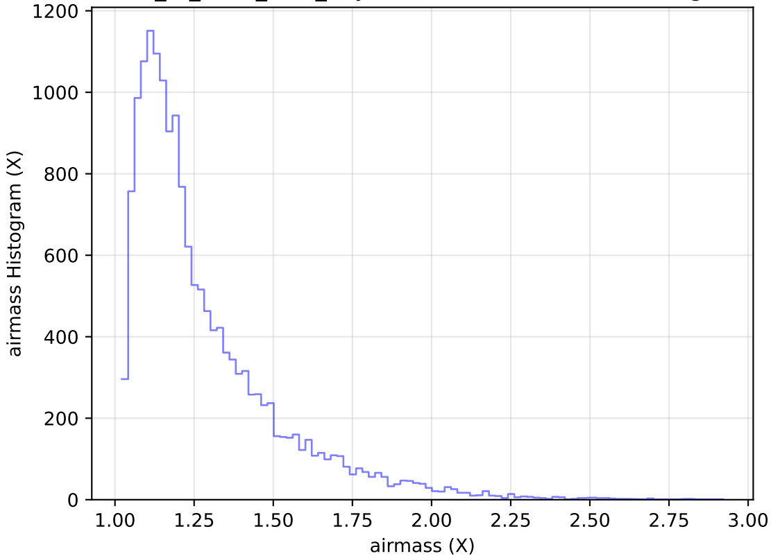
extra_ss_neo4_v3.4_10yrs Yr 1 u band: airmass Histogram
