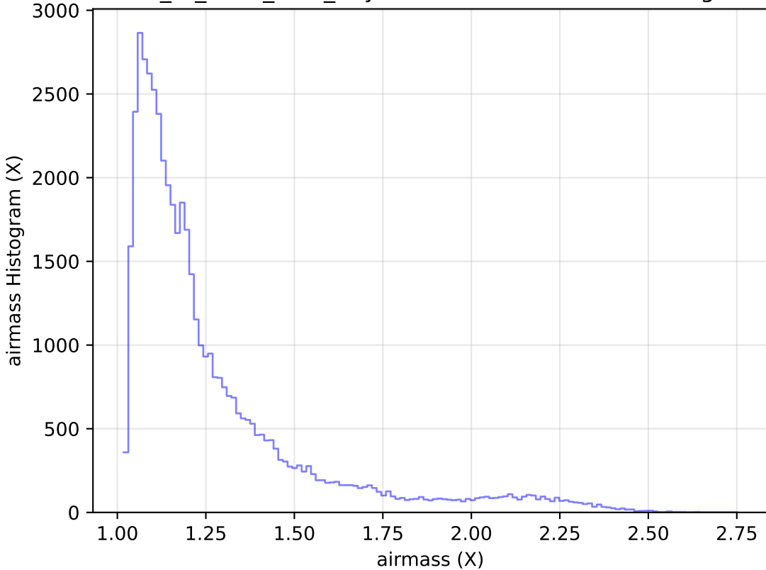
extra_ss_neo4_v3.4_10yrs Yr 1 r band: airmass Histogram
