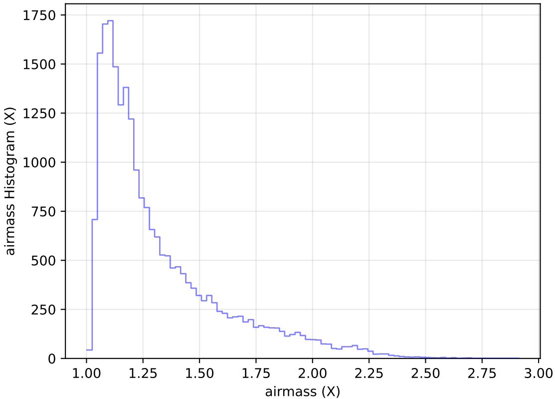
extra_ss_neo4_v3.4_10yrs Yr 1 g band: airmass Histogram
