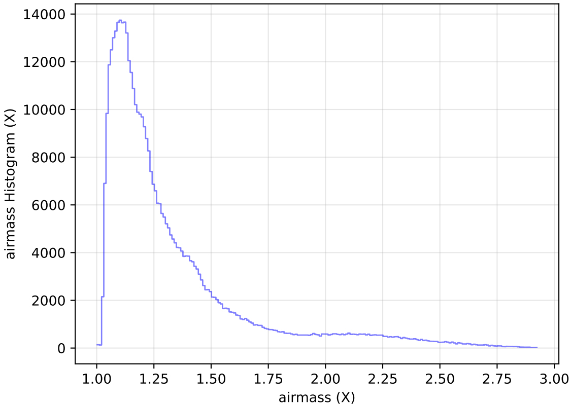
extra_ss_neo4_v3.4_10yrs WFD z band: airmass Histogram
