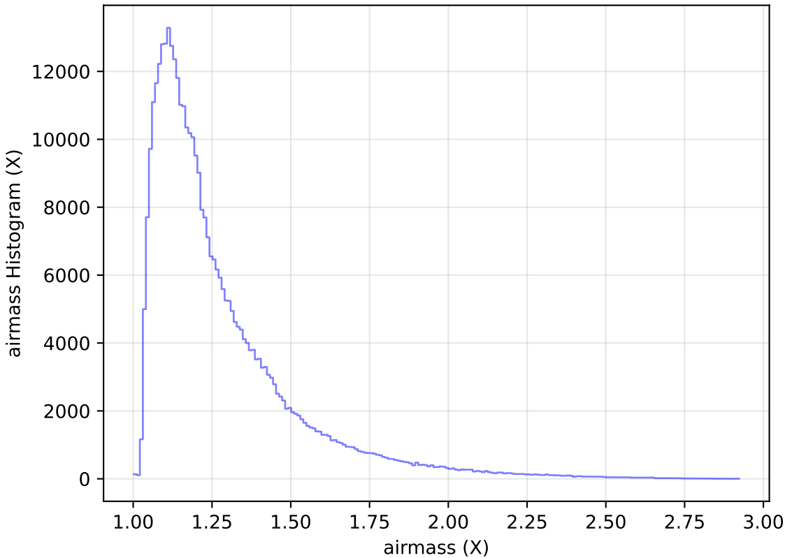
extra_ss_neo4_v3.4_10yrs WFD y band: airmass Histogram
