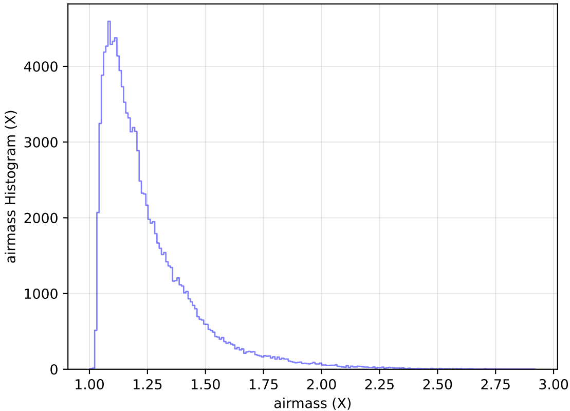
extra_ss_neo4_v3.4_10yrs WFD u band: airmass Histogram
