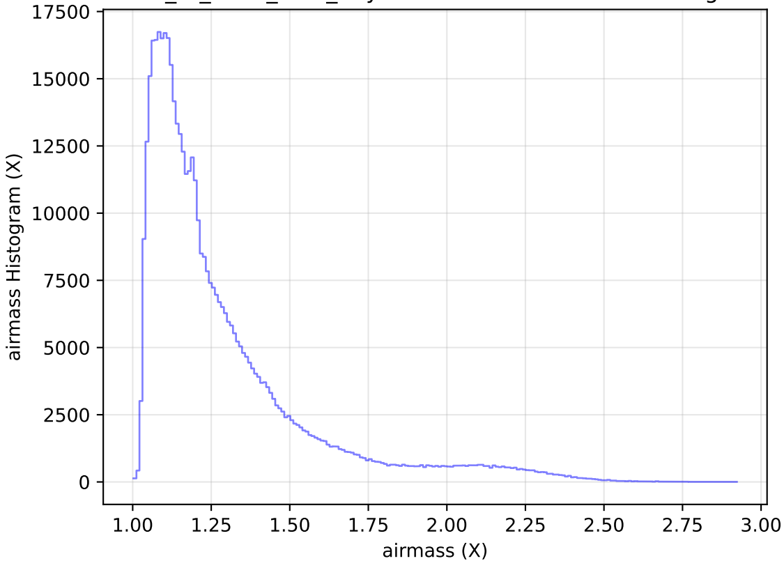
extra_ss_neo4_v3.4_10yrs WFD r band: airmass Histogram
