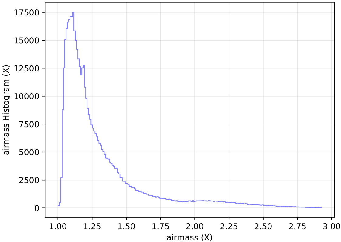
extra_ss_neo4_v3.4_10yrs WFD i band: airmass Histogram
