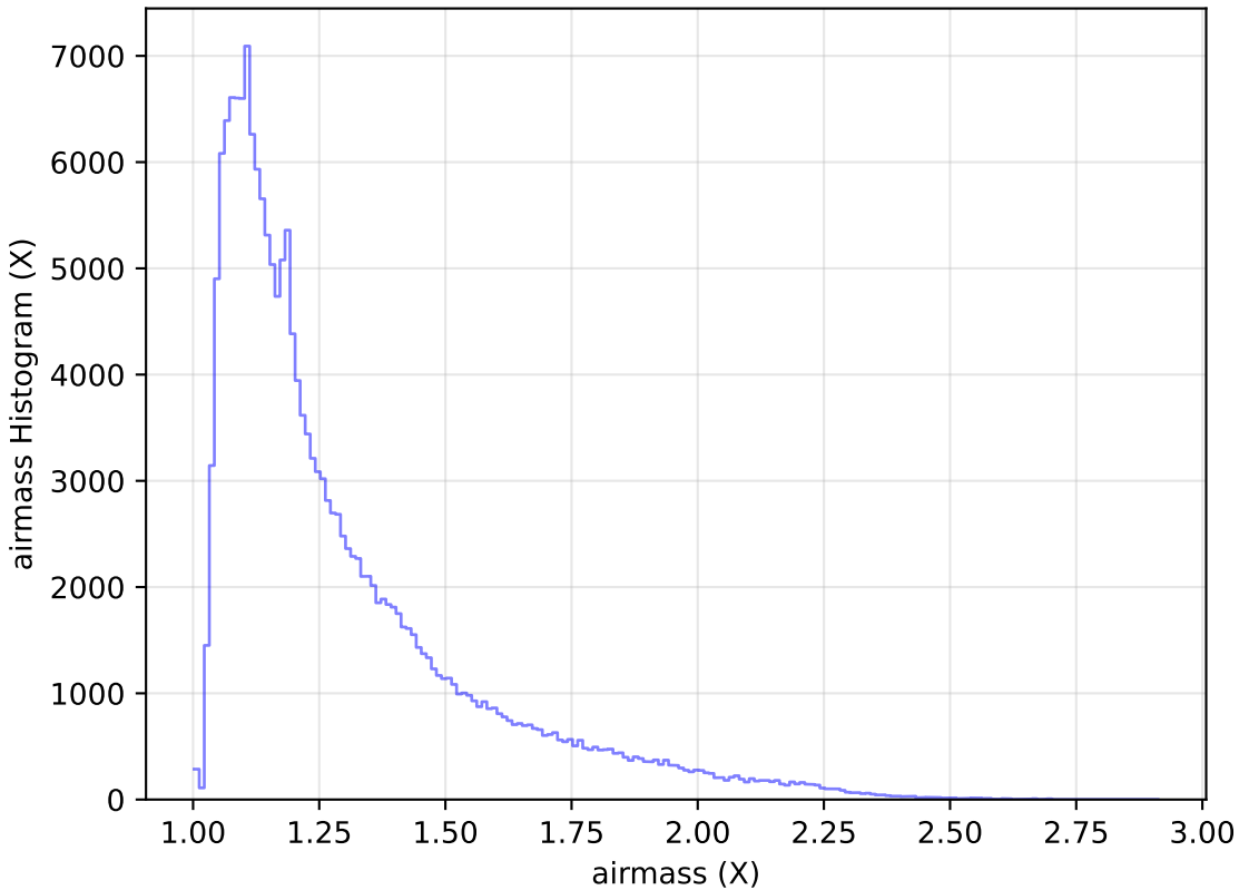
extra_ss_neo4_v3.4_10yrs WFD g band: airmass Histogram
