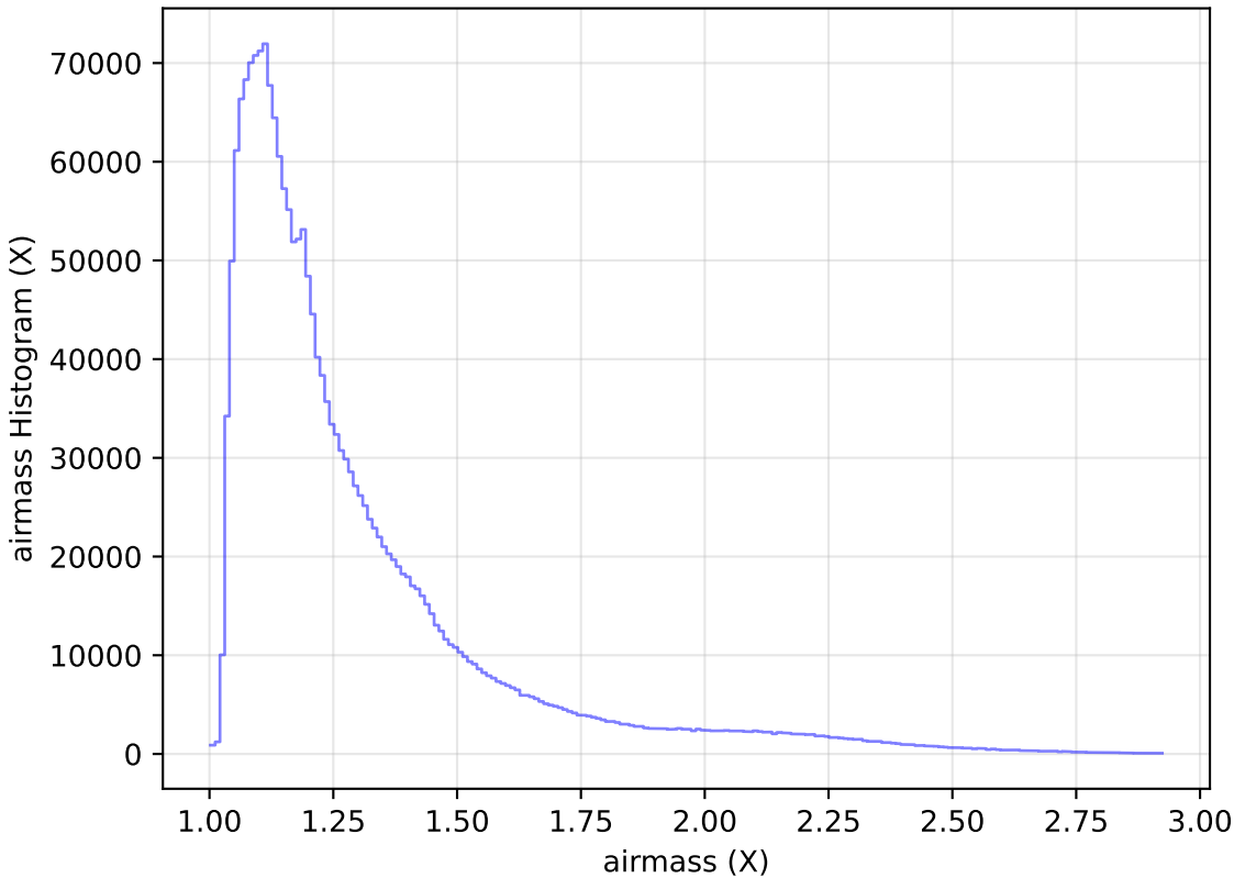
extra_ss_neo4_v3.4_10yrs WFD all bands: airmass Histogram
