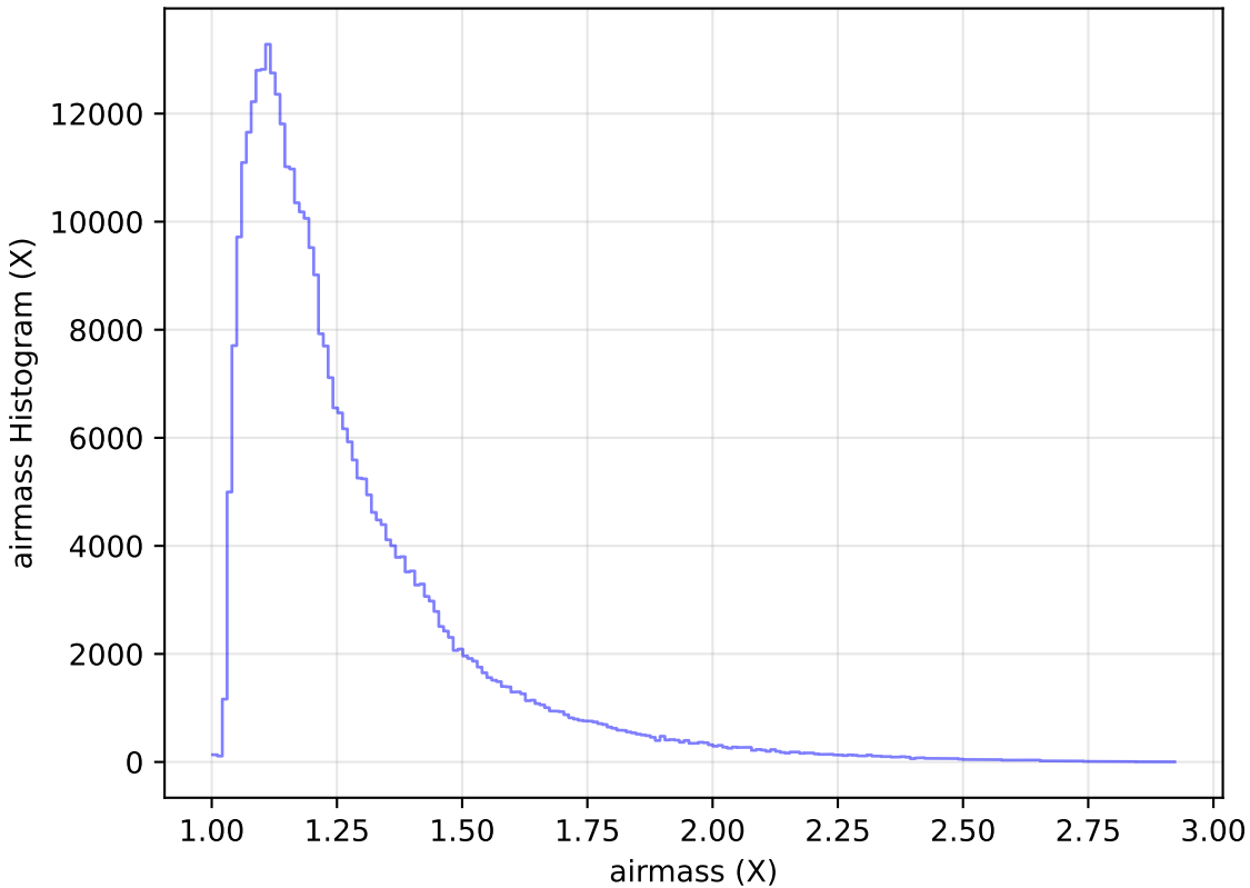
extra_ss_neo4_v3.4_10yrs All sky y band: airmass Histogram
