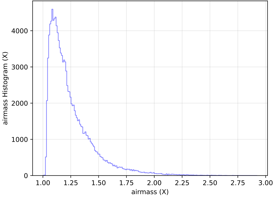
extra_ss_neo4_v3.4_10yrs All sky u band: airmass Histogram
