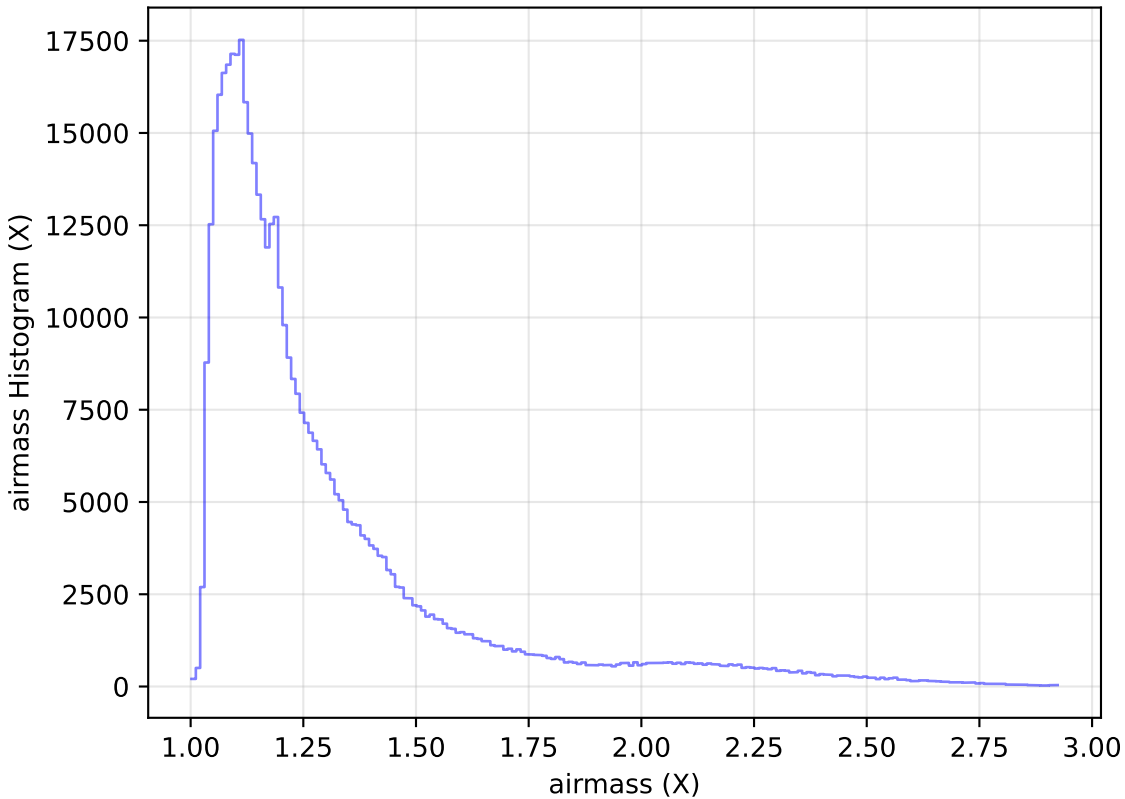
extra_ss_neo4_v3.4_10yrs All sky i band: airmass Histogram
