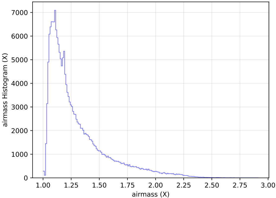
extra_ss_neo4_v3.4_10yrs All sky g band: airmass Histogram
