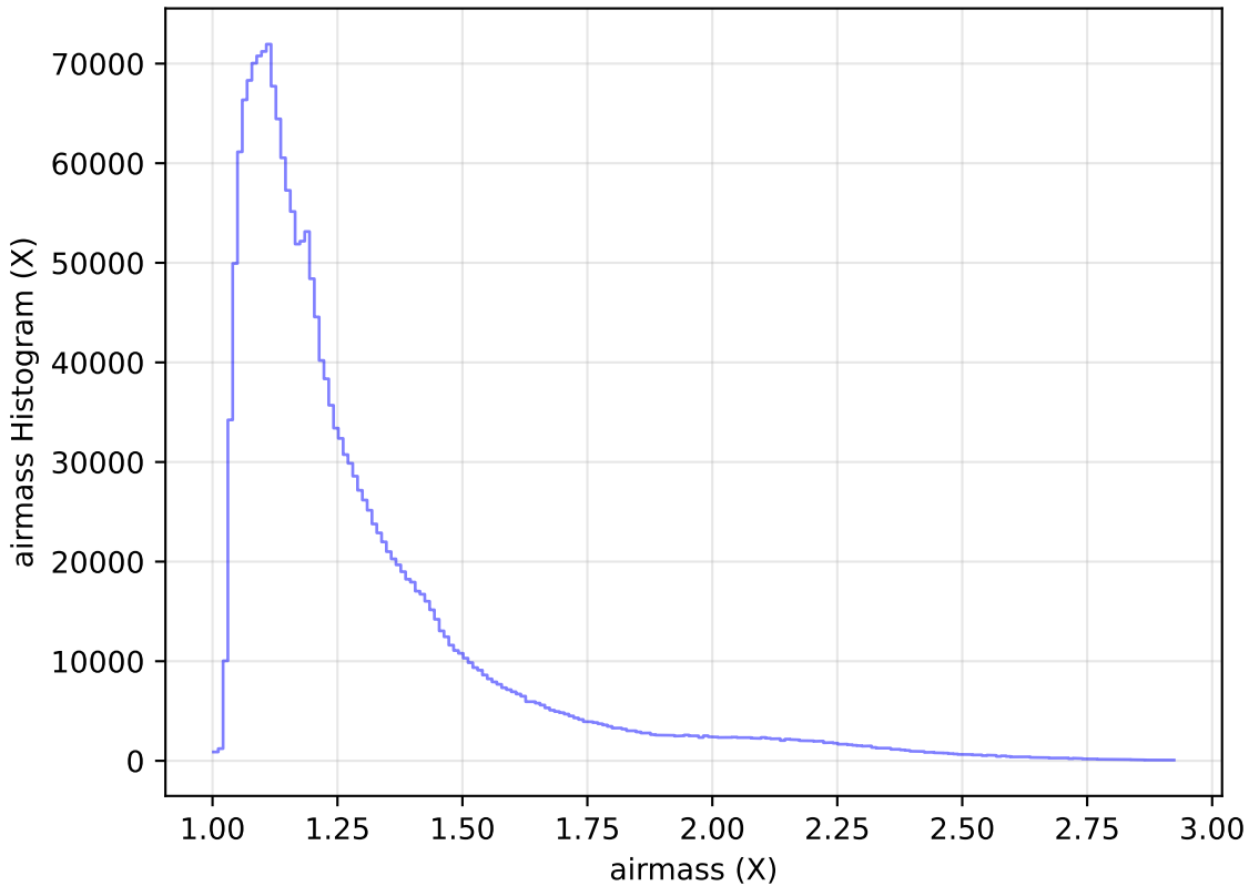
extra_ss_neo4_v3.4_10yrs All sky all bands: airmass Histogram
