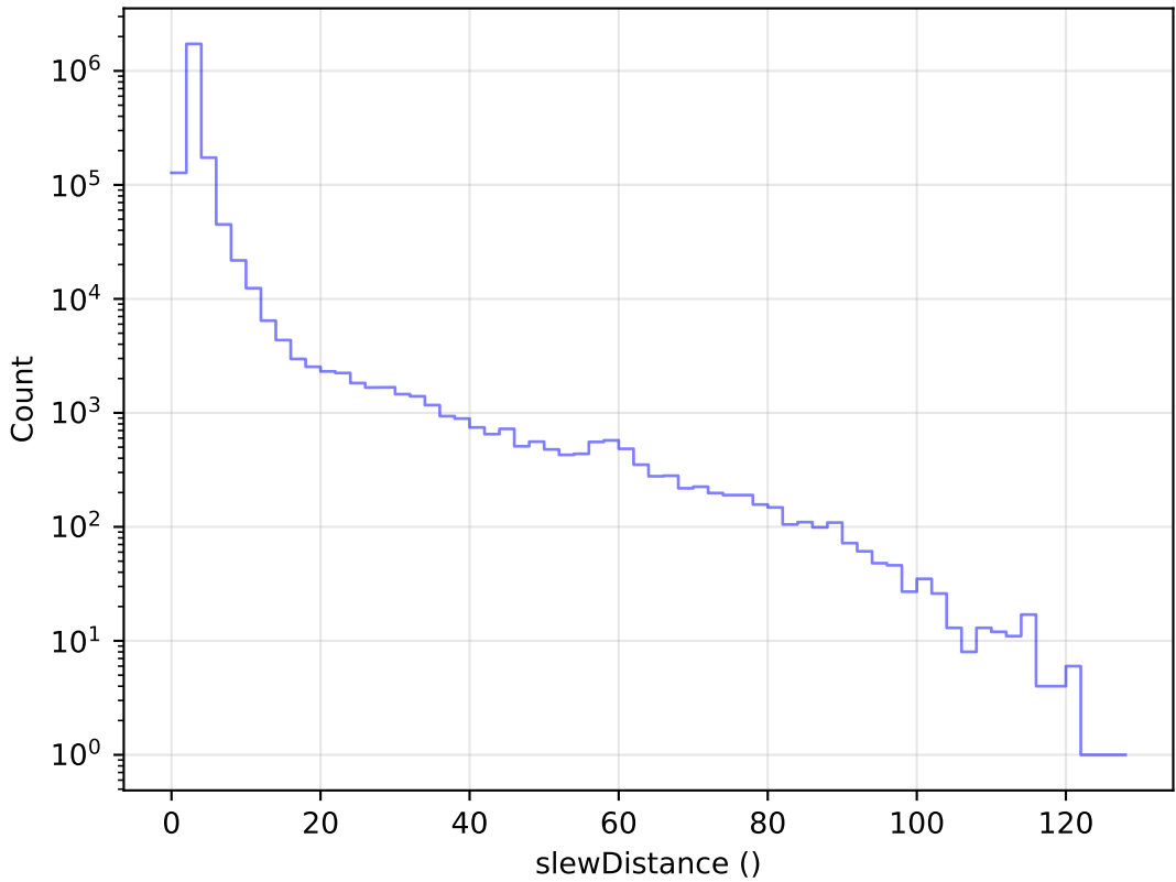
extra_ss_neo4_v3.4_10yrs All visits: Slew Distance Histogram
