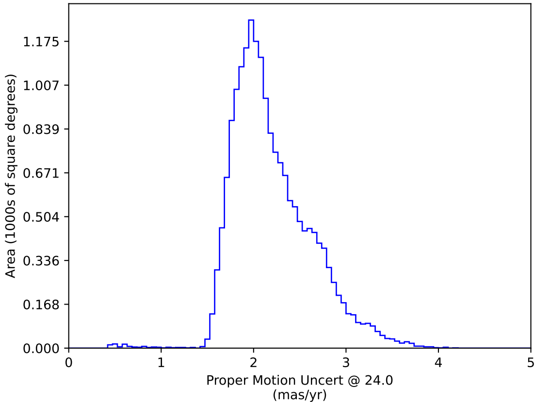
extra_ss_neo4_v3.4_10yrs WFD: Proper Motion Uncert @ 24.0
