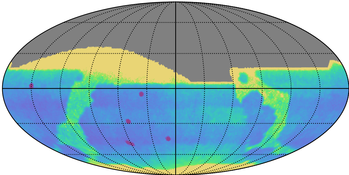
extra_ss_neo4_v3.4_10yrs All sky: Proper Motion Uncert @ 24.0
