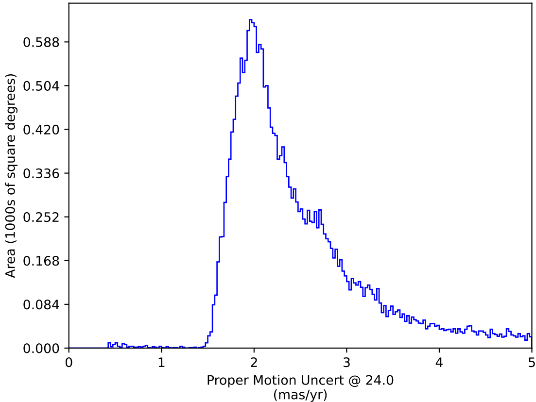
extra_ss_neo4_v3.4_10yrs All sky: Proper Motion Uncert @ 24.0
