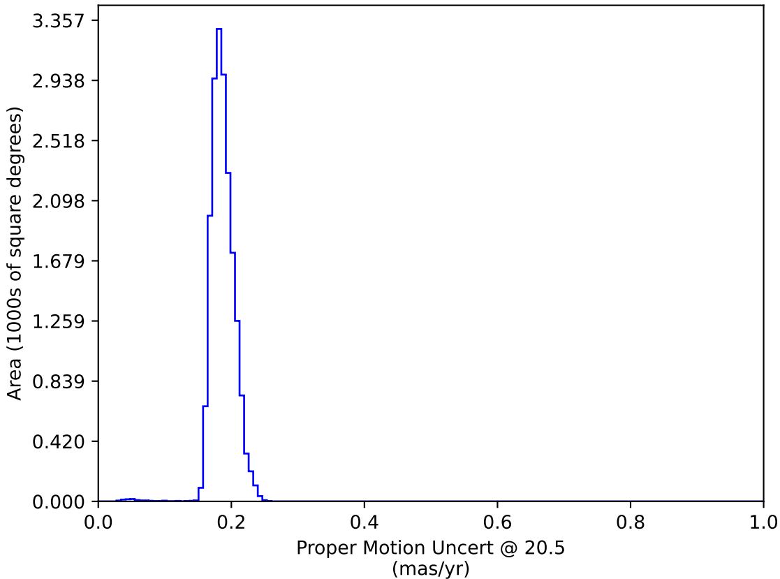
extra_ss_neo4_v3.4_10yrs WFD: Proper Motion Uncert @ 20.5
