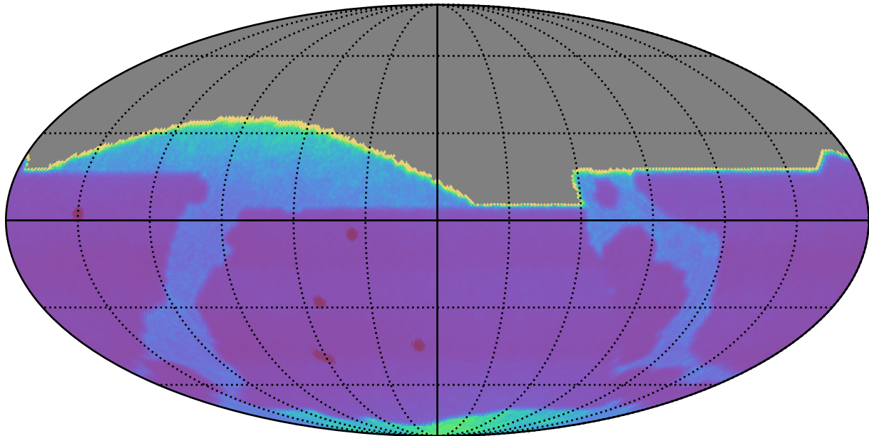
extra_ss_neo4_v3.4_10yrs All sky: Proper Motion Uncert @ 20.5
