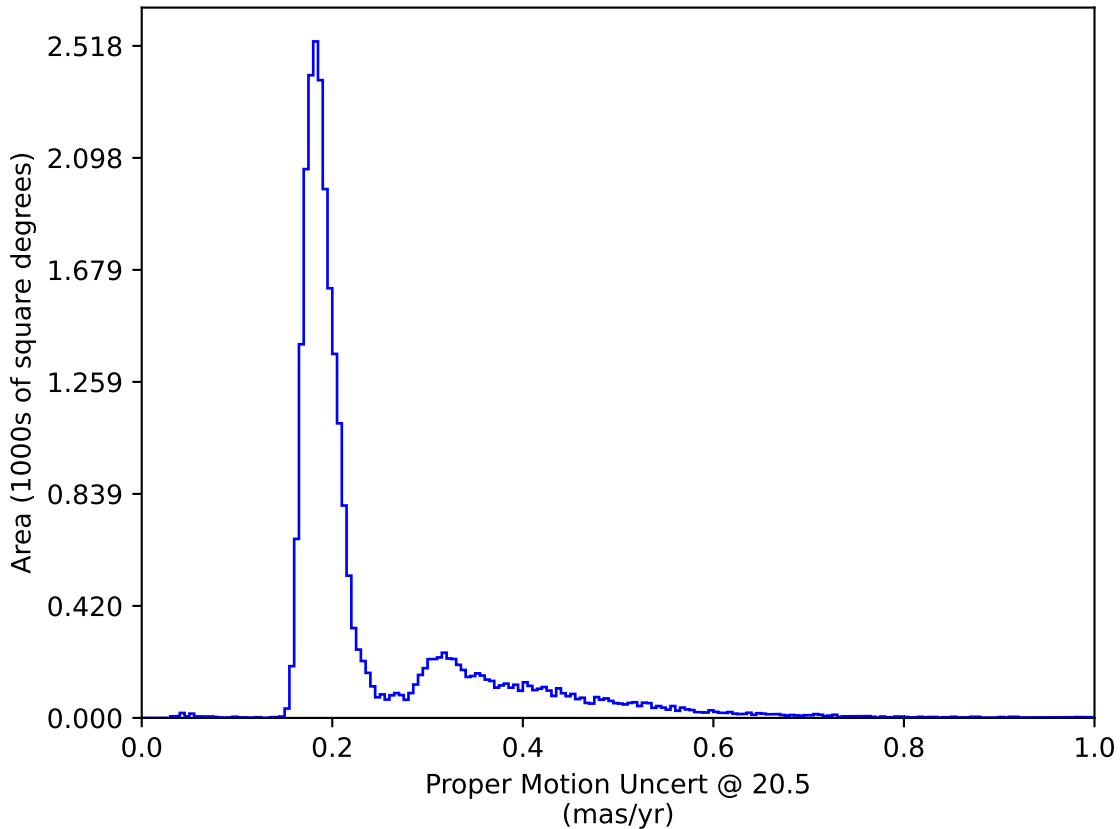
extra_ss_neo4_v3.4_10yrs All sky: Proper Motion Uncert @ 20.5
