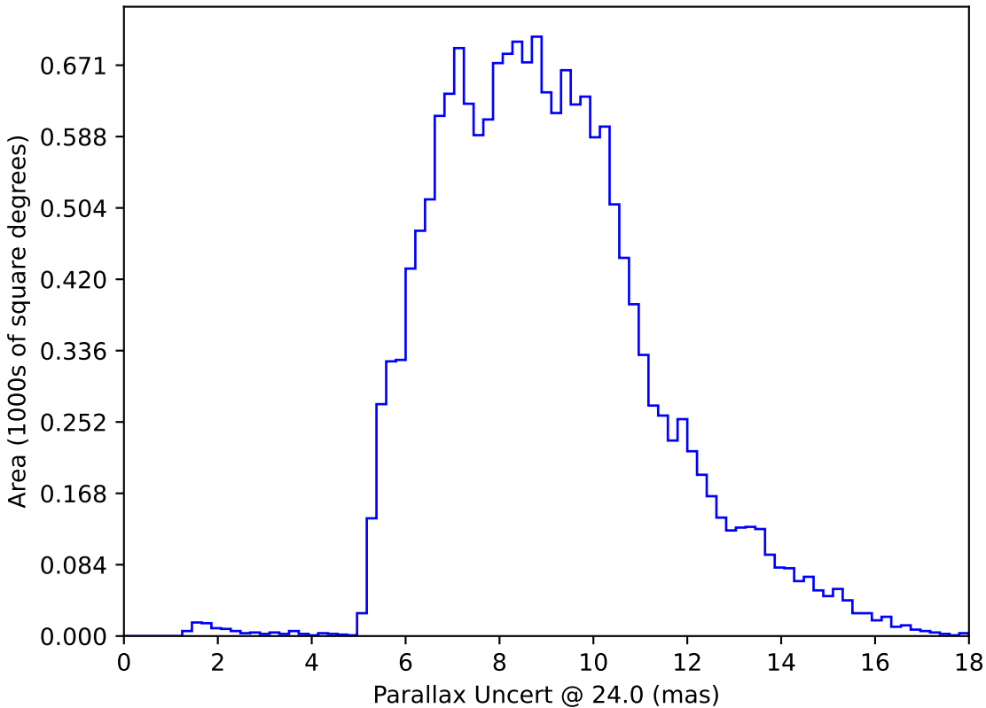
extra_ss_neo4_v3.4_10yrs WFD: Parallax Uncert @ 24.0
