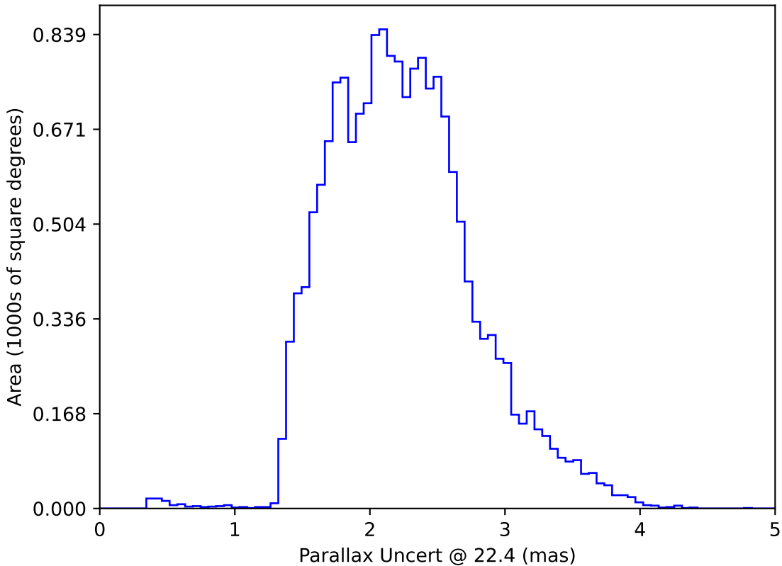
extra_ss_neo4_v3.4_10yrs WFD: Parallax Uncert @ 22.4
