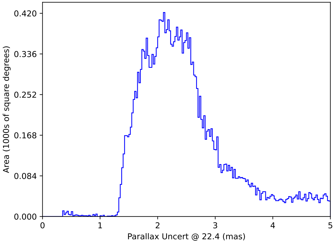
extra_ss_neo4_v3.4_10yrs All sky: Parallax Uncert @ 22.4
