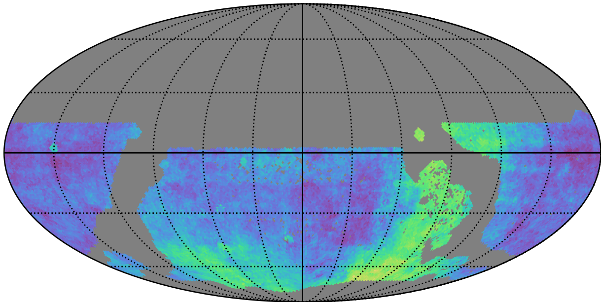
extra_ss_neo4_v3.4_10yrs WFD: Parallax Coverage @ 24.0
