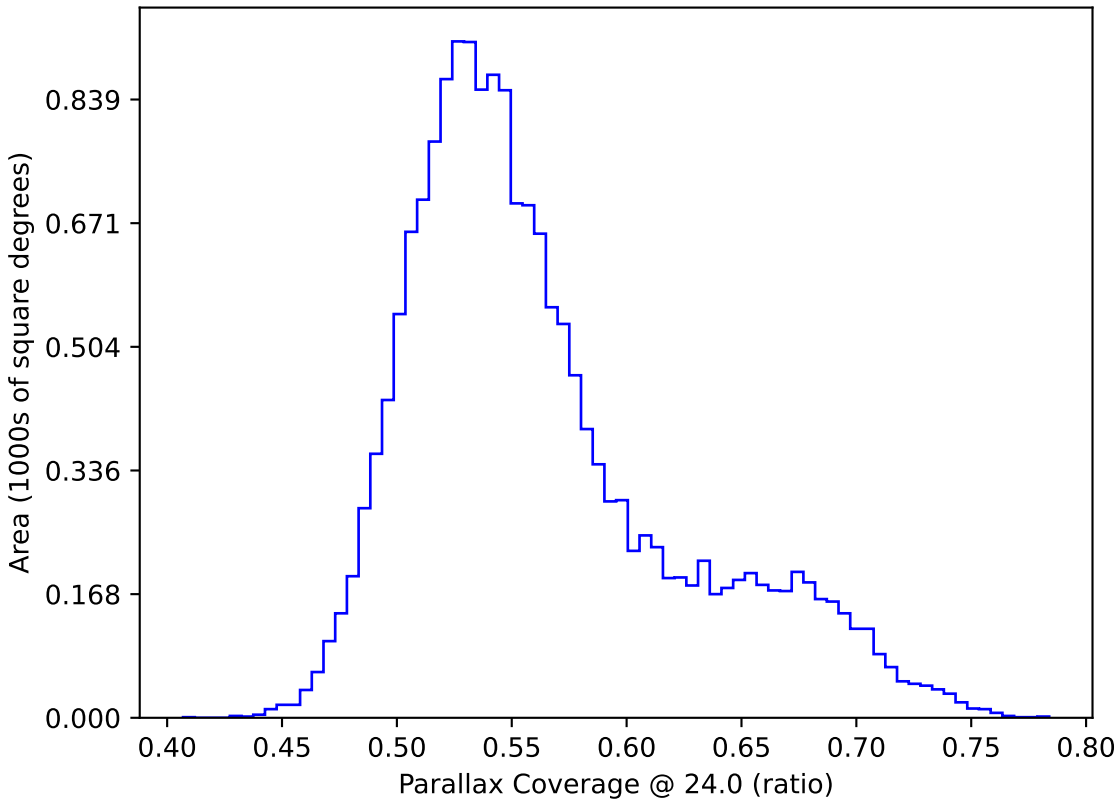
extra_ss_neo4_v3.4_10yrs WFD: Parallax Coverage @ 24.0
